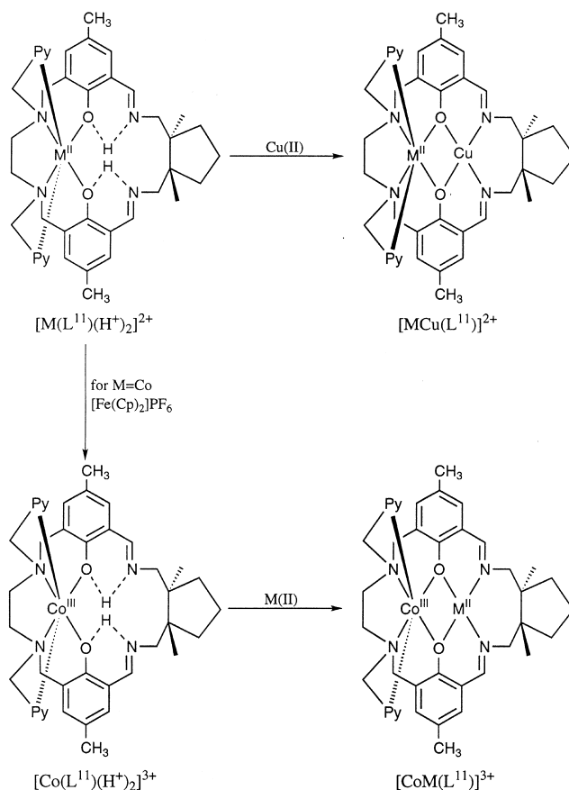
Scheme 6. Site-selective synthesis of M^{II}Cu^{II} and Co^{III}M^{II} complexes of L^{11}
