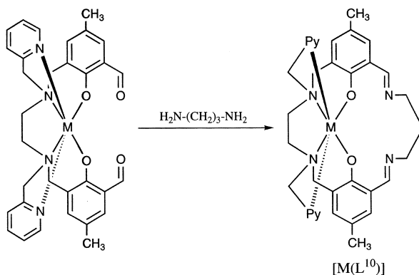
Scheme 5. Template synthesis of [M(L^{10})] .
